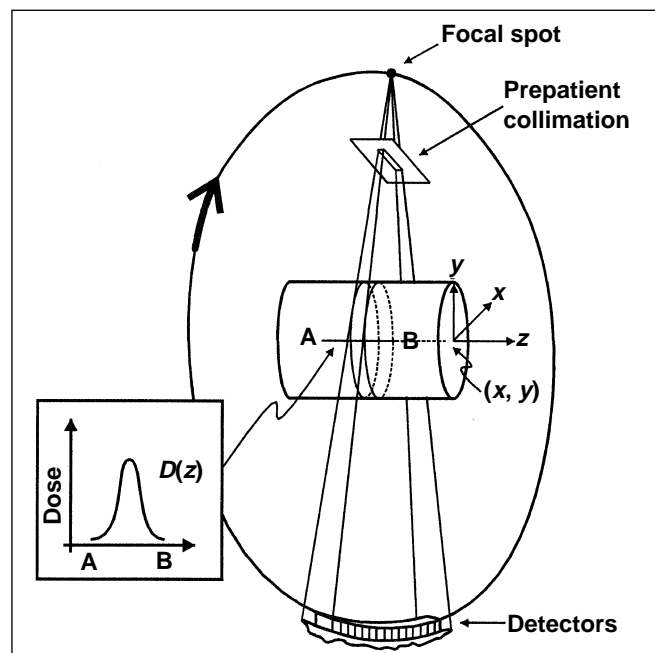
Fig. 1.—Illustration of CT system geometry shows intersection of X-ray beam with dosimetry phantom. Insert indicates idealized dose profile measured along line AB. (Courtesy of Shope TB, Food and Drug Administration's Center for Devices and Radiological Health, Gaithersburg, MD)
