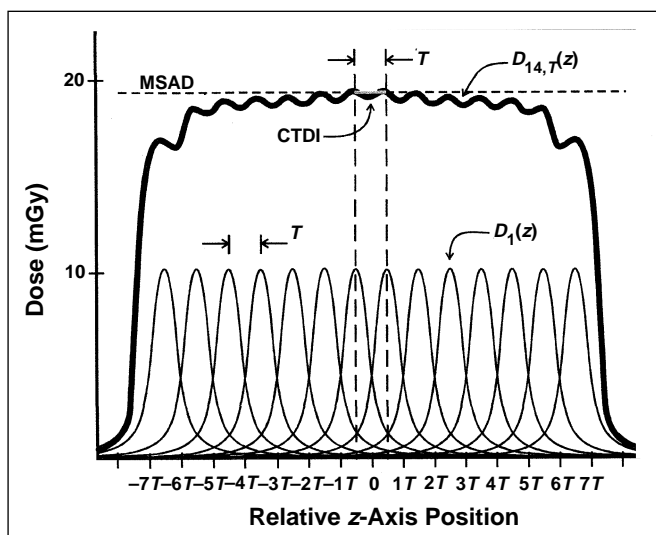
Fig. 2.—Illustration of multiple scan dose profile shows results from series of 14 scans with increment equal to slice thickness ( T ). Multiple scan average dose (MSAD) is given by CT dose index (CTDI) indicated at central portion of multiple scan dose profile. (Courtesy of Shope TB, Food and Drug Administration's Center for Devices and Radiological Health, Gaithersburg, MD)
