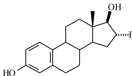
Figure 3.1. 16- \alpha -[ 18 F]fluoro-17- \beta -fluoroestradiol
