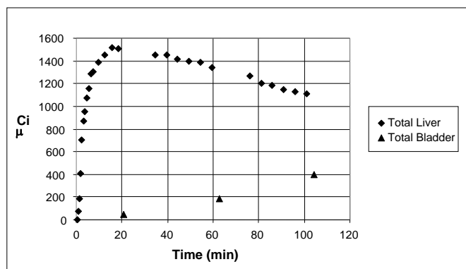
Figure 5.3. Total liver and bladder activity as a function of time after FES injection for a patient injected with an approximately 6,000 \mu Ci (6 mCi) total dose. 14
