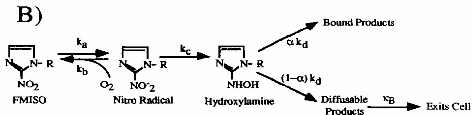
Figure 2. Metabolism of 2-nitroimidazoles. See text (above figure) for further details
